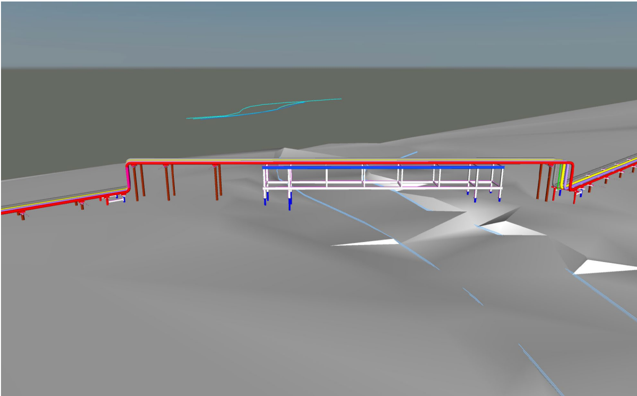
Figure 2: Model view of the pipeline infrastructure crossing
