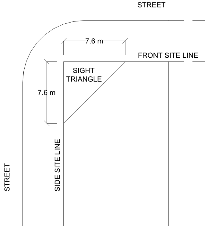
Figure 2-2: Sight Triangle
