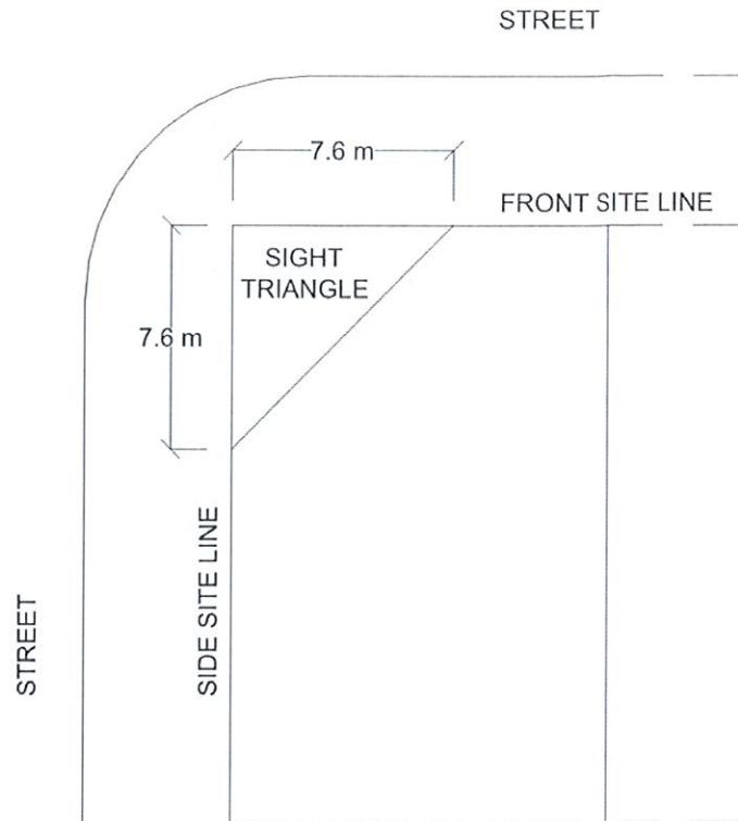
Figure 2-2: Sight Triangle
